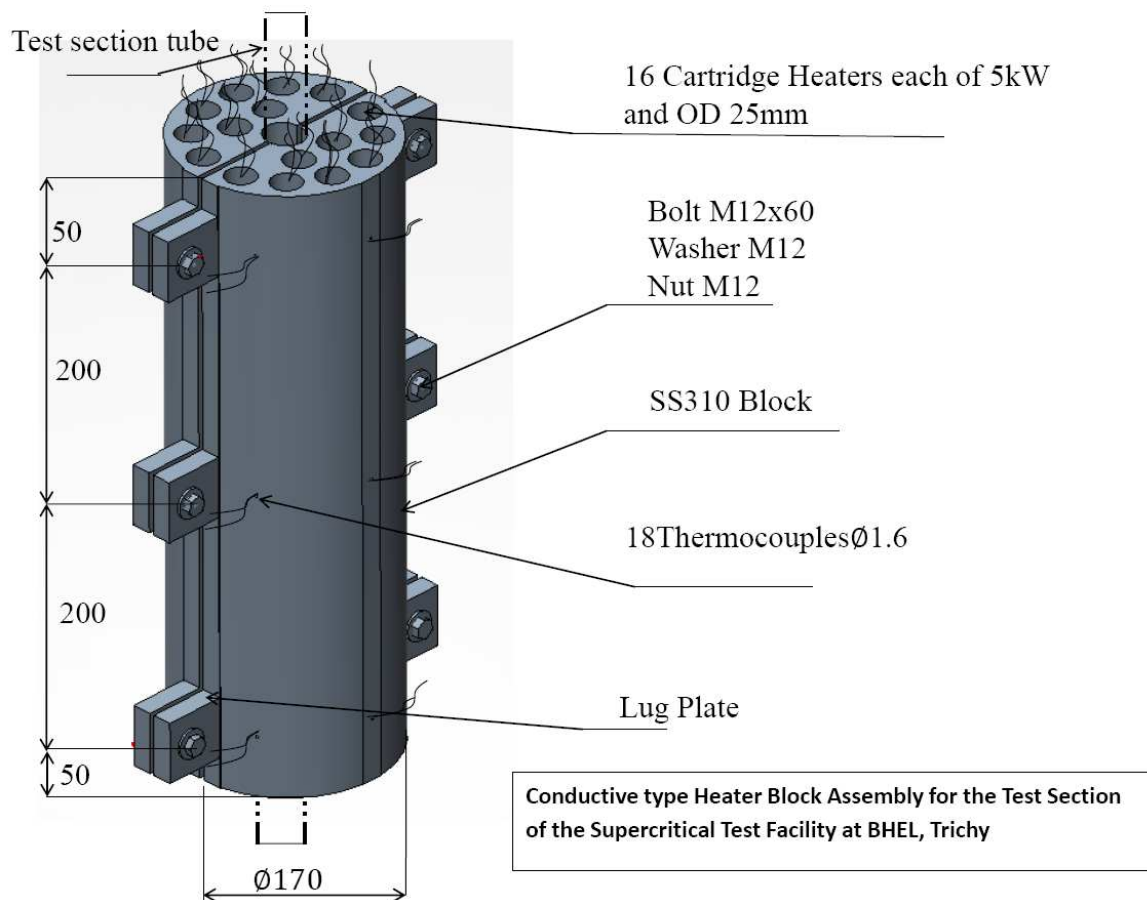
Fig 01: Heater Block
