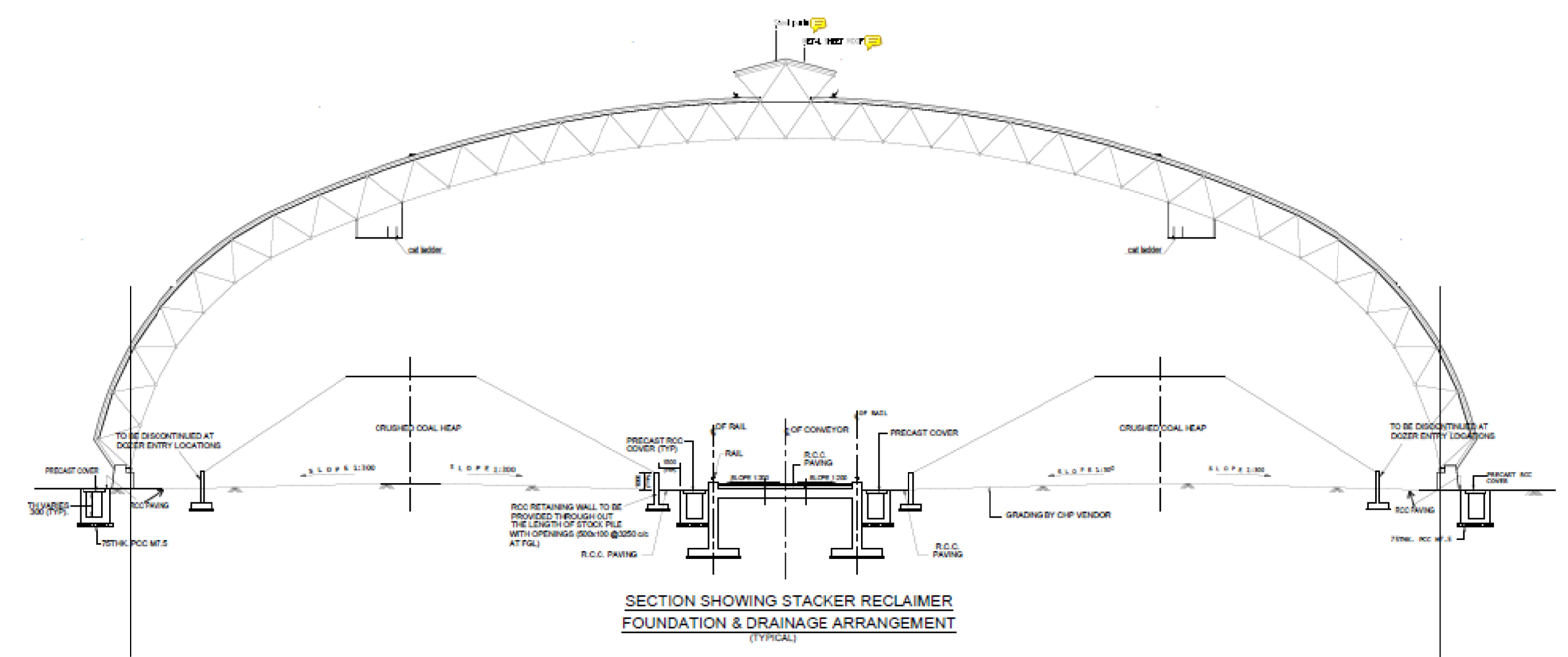
VIEW Q-Q Civil to also refer the Cross section furnished by customer in Spec. PART - 5
