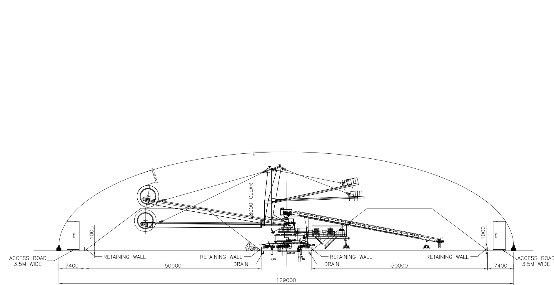
VIEW Q-Q COAL STOCKPILE SHED
