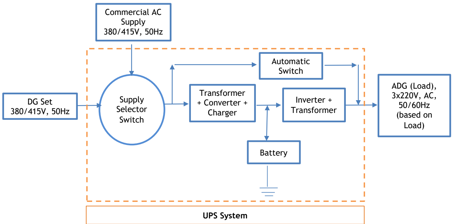
Representative Block Diagram of Power Supply Unit
