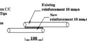
TYPICAL DETAIL OF X
