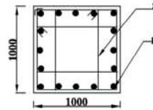
SECTION ON BB PEDESTAL (EXISTING) SCALE:1:50
