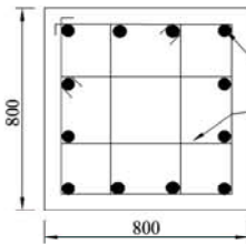
SECTION ON BB PEDESTAL
