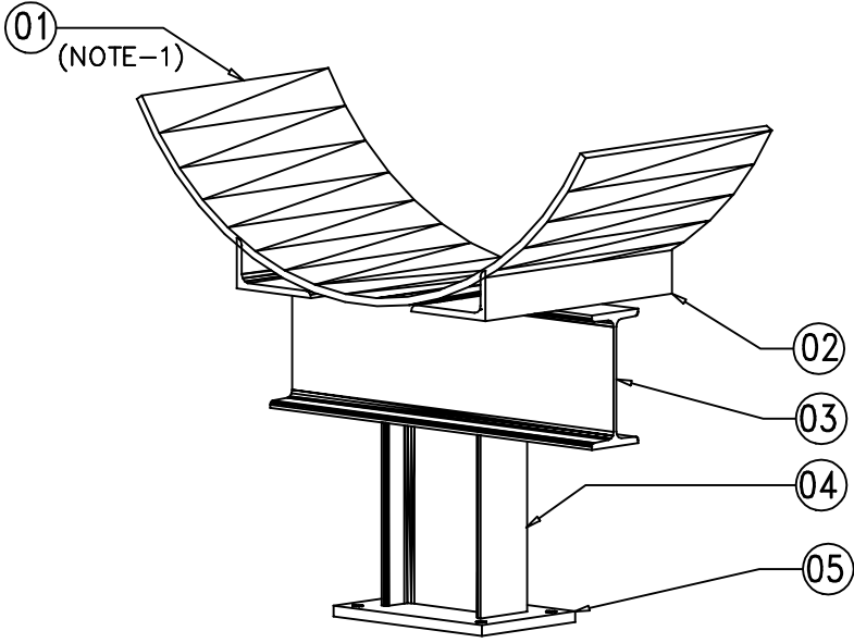
ISOMETRIC VIEW ( FOR REF. ONLY )
