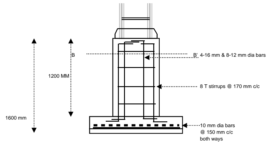
REINFORCEMENT DETAILS
