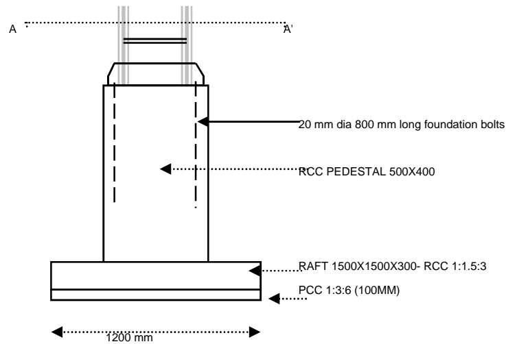
COLUMN FOOTING/PEDESTAL
