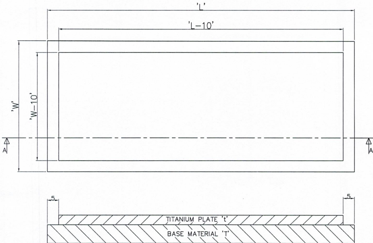
SECTION-AA
