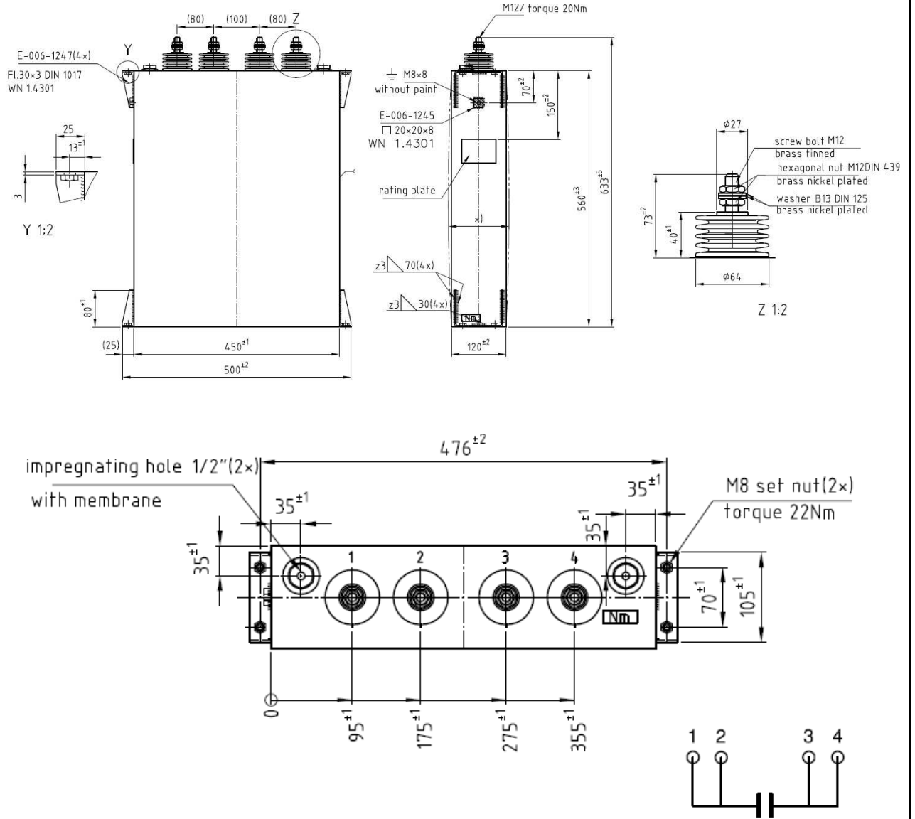
Fig 2: Dimensional Drawing
