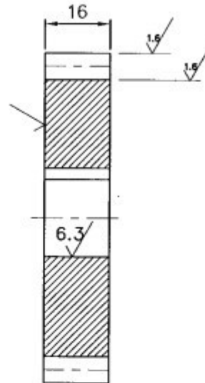
SECTION EE
