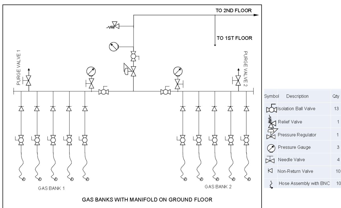
Manifold Layout No.- 1
