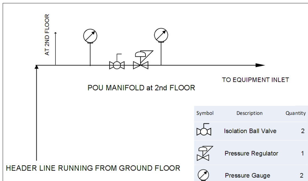
Manifold Layout No.- 2
