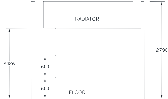
SECTIONAL ELEVATION
