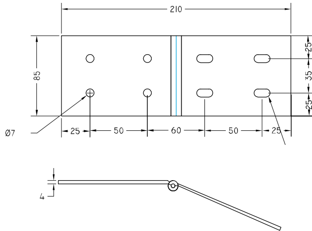
FRP ADJUSTABLE HORIZONTAL SPLICE PLATE
