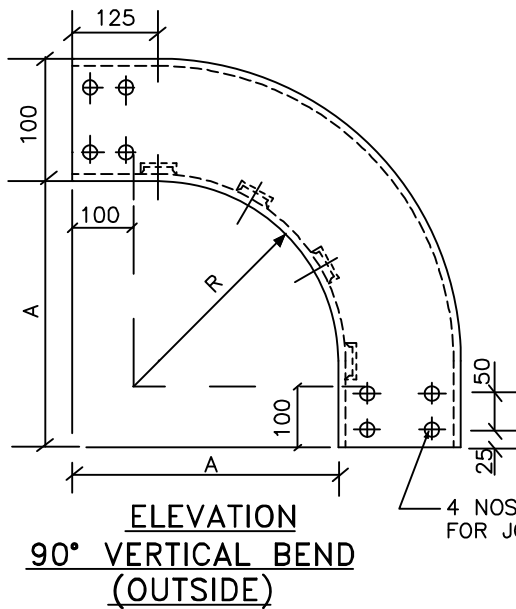
90° VERTICAL BEND (OUTSIDE)
